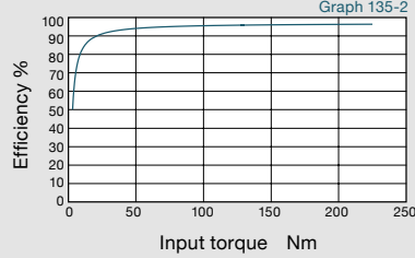
Reduction ratio = 10
