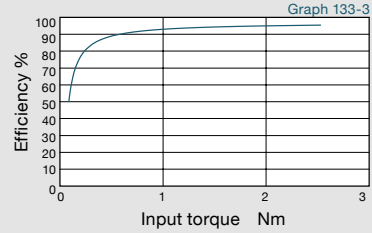
Reduction ratio = 20
