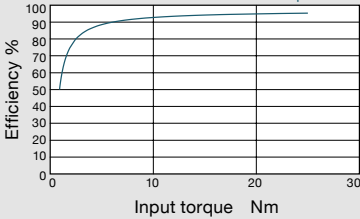
Reduction ratio = 31
