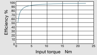
Reduction ratio = 13
