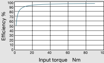
Reduction ratio = 10
