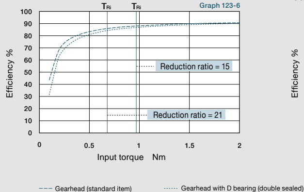
Reduction Ratio = 15, 21
