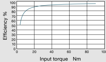
Reduction ratio = 7
