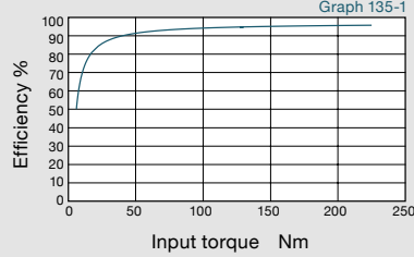
Reduction ratio = 7
