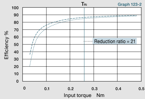
Reduction Ratio = 21
